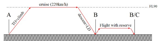
Fig. 5. Mission profile derived from operational concept
